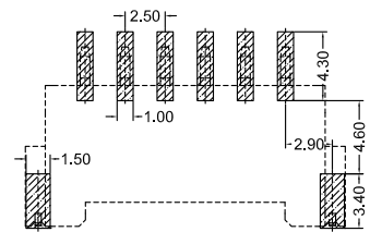
Recommended P.C.B Layout General Tolerance±0.05
