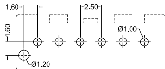
Recommended P.C.B Layout General Tolerance±0.05
