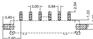
Recommended P.C.B Layout General Tolerance±0.05
