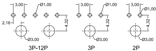
Recommended P.C.B Layout General Tolerance±0.05
