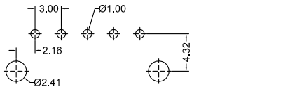
Recommended P.C.B Layout General Tolerance±0.05
