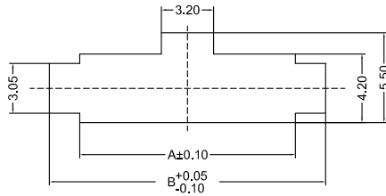
SINGLE ROW RECOMMENDED PANEL CUT-OUT (DESIGNED FOR 1.57mm TO 2.30mm THICK STAMPED PANEL OR PRINTED CIRCUIT BOARD)
