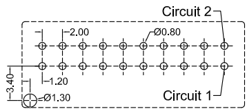
Recommended P.C.B Layout General Tolerance±0.05
