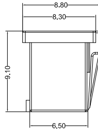
8P~14P Without Guide bulge 16P~40P With Guide bulge Scale: 1/0.8
