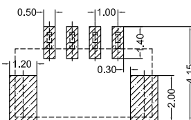
Recommended P.C.B Layout General Tolerance±0.05
