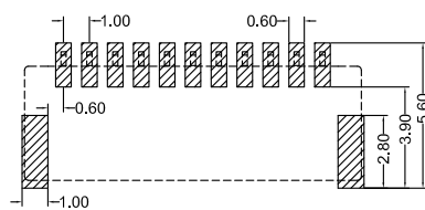
Recommended P.C.B Layout General Tolerance±0.05
